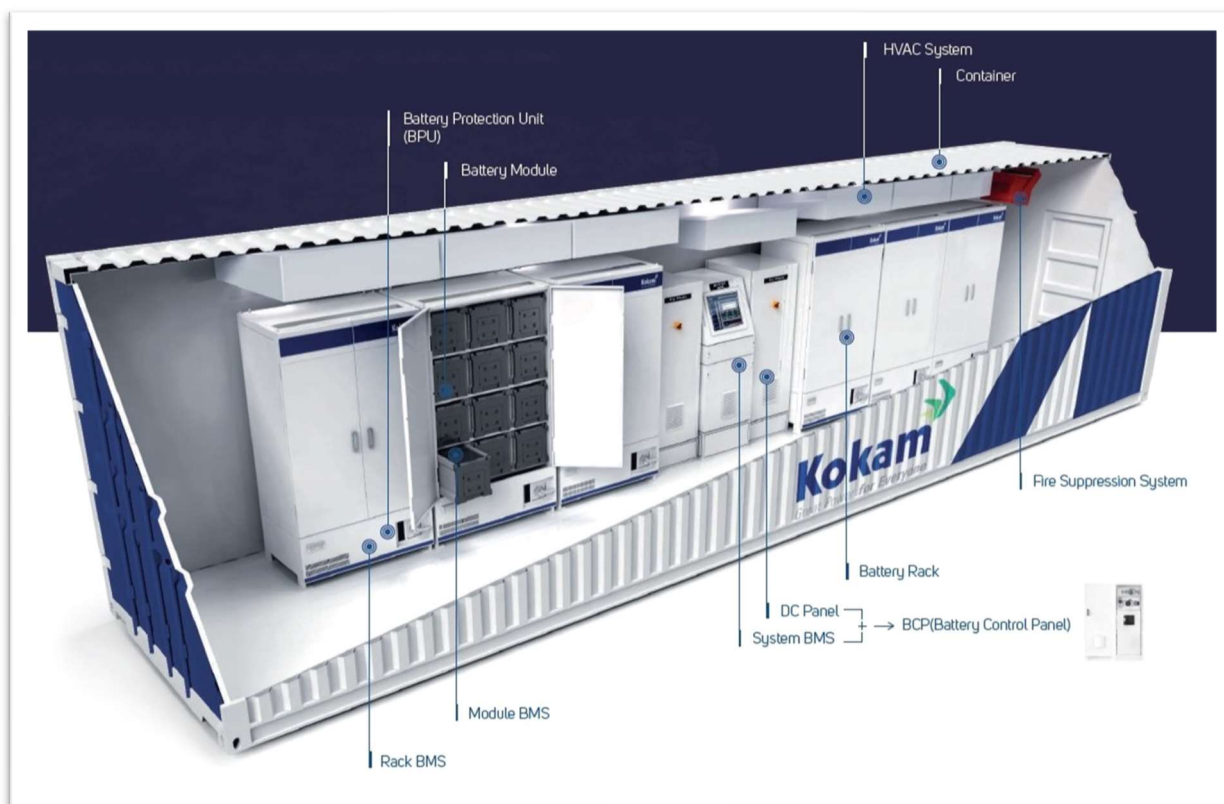
Figura 3 - Container Storage
