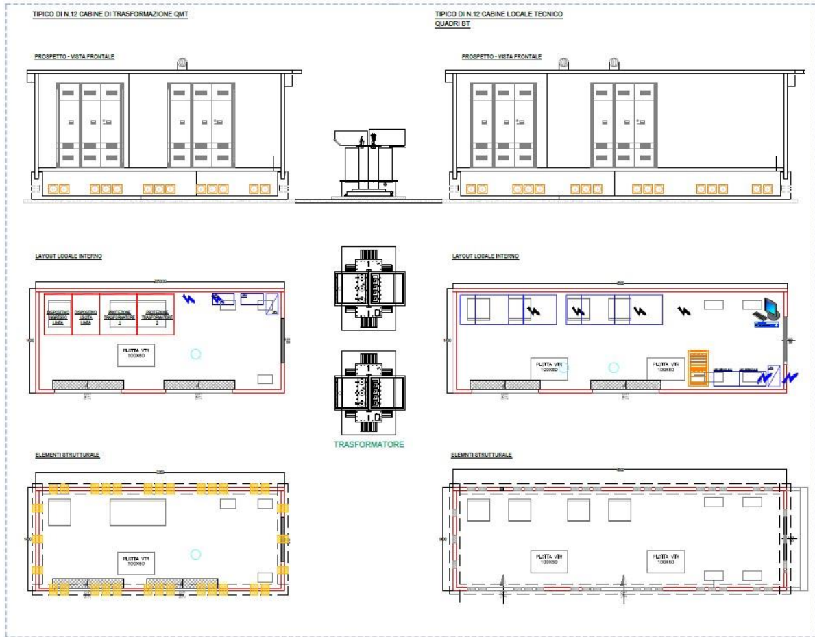
Figura 2.1: Power Station
