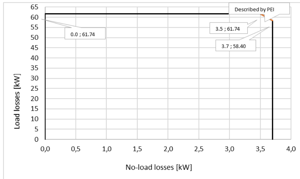
Figure 4-1: Transformer losses allowable area for 7000kVA variant
