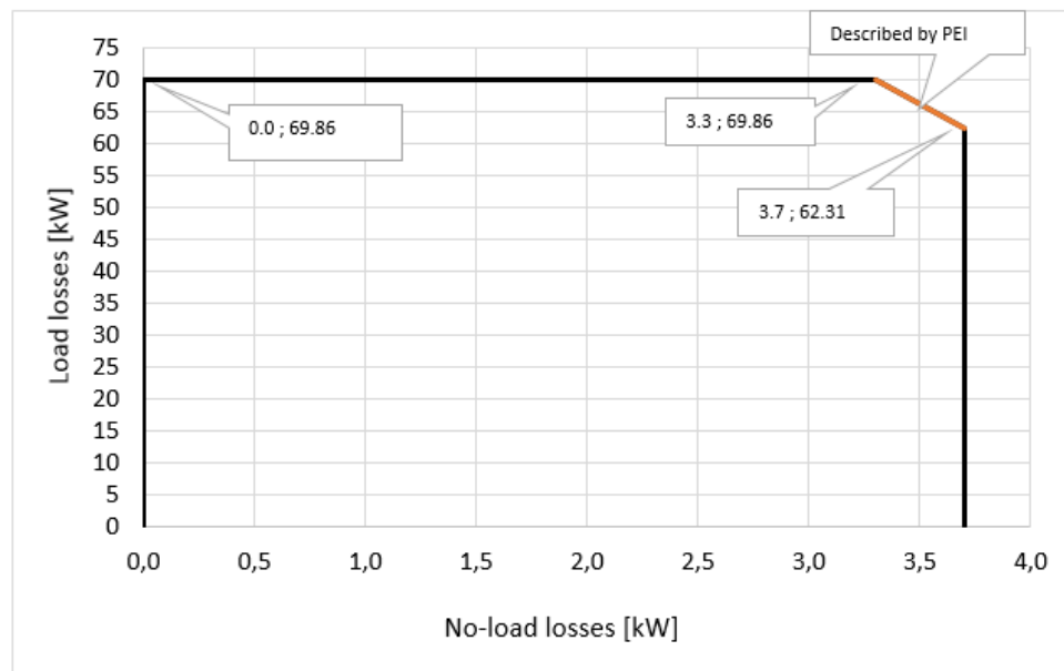
Figure 4-2: Transformer losses allowable area for 7300kVA variant
