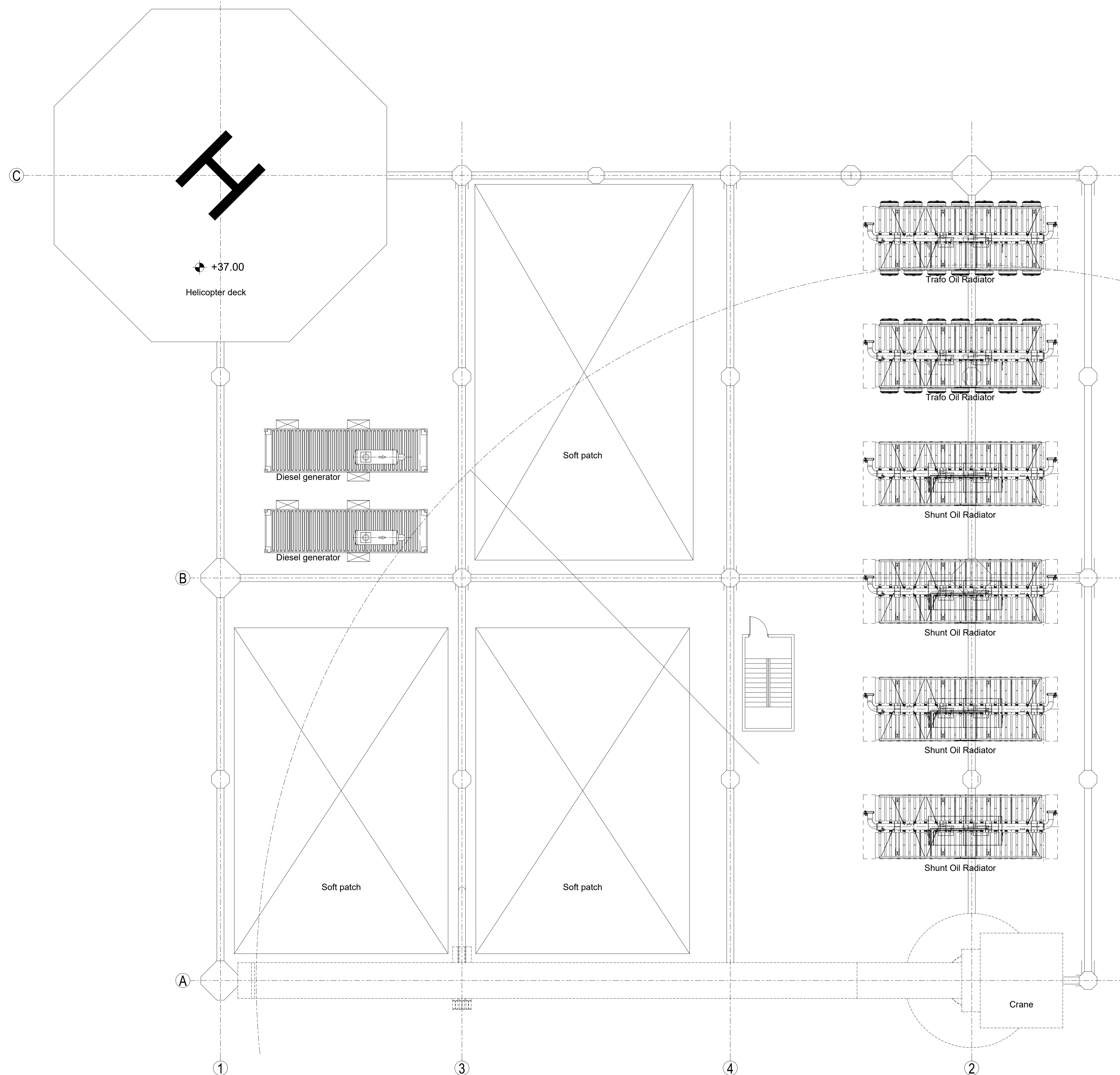
PLAN AT EL. +34.00
