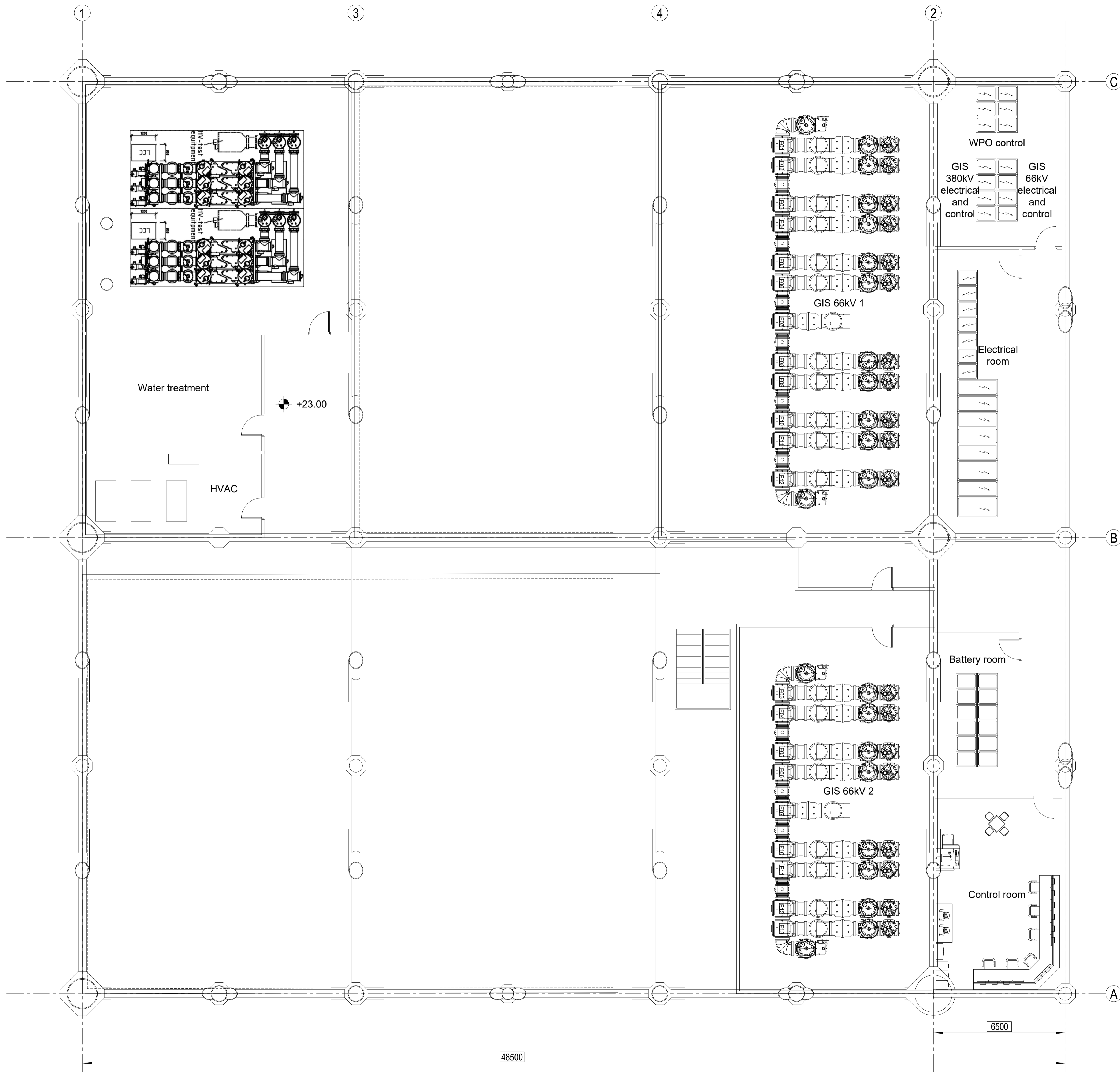
PLAN AT EL. +23.00
