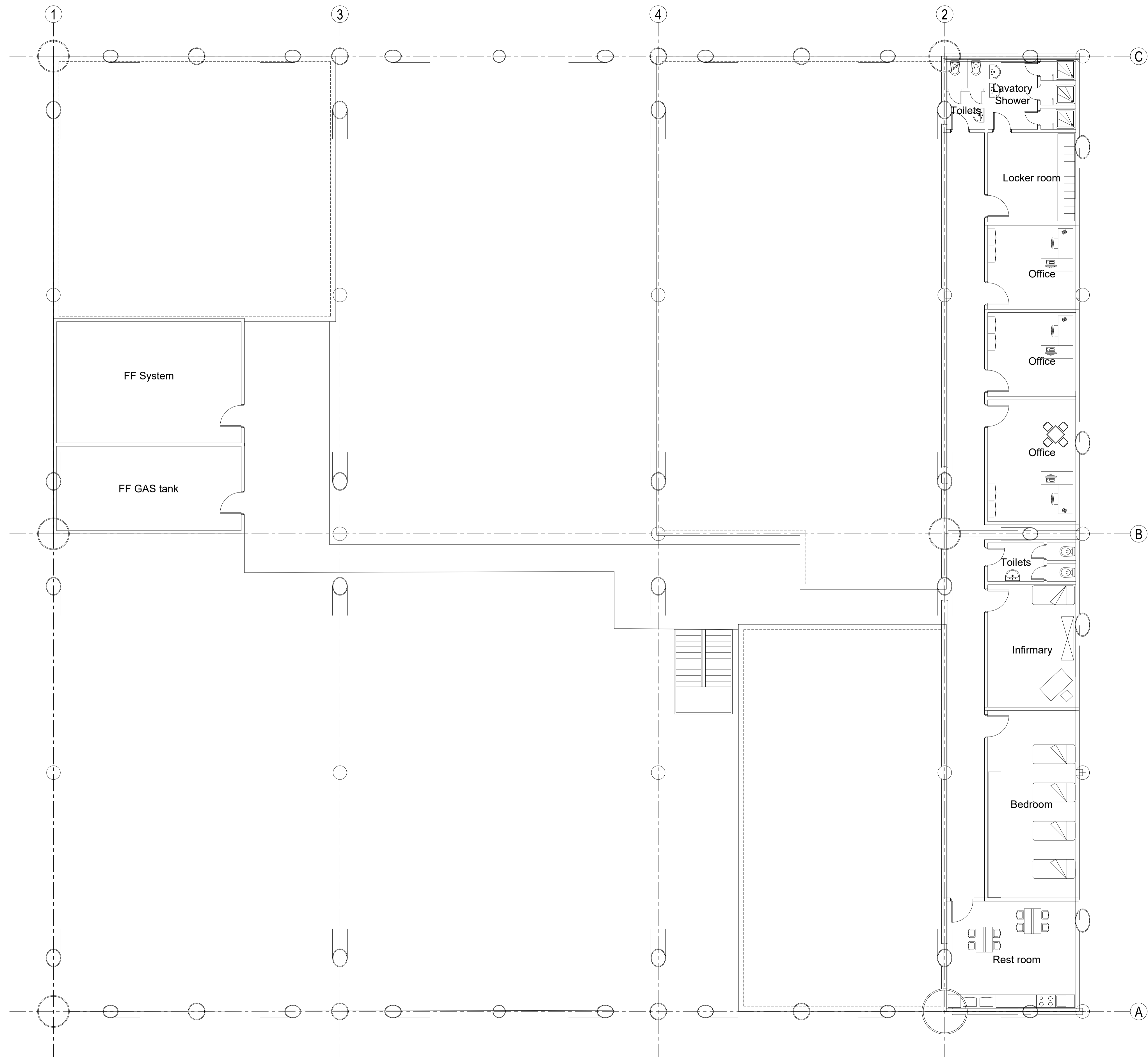
PLAN AT EL. +28.60
