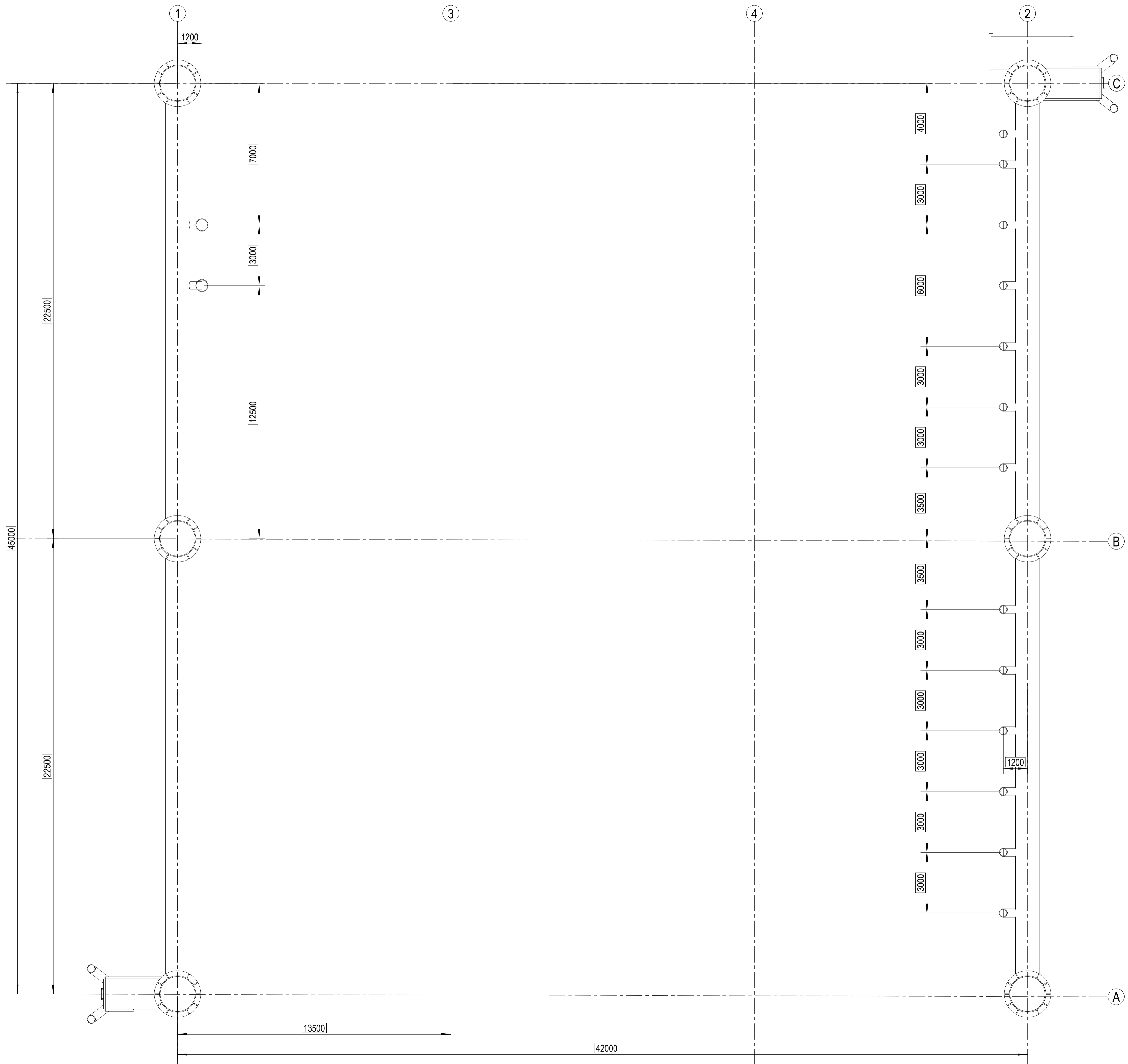
PLAN AT EL. +12.00
