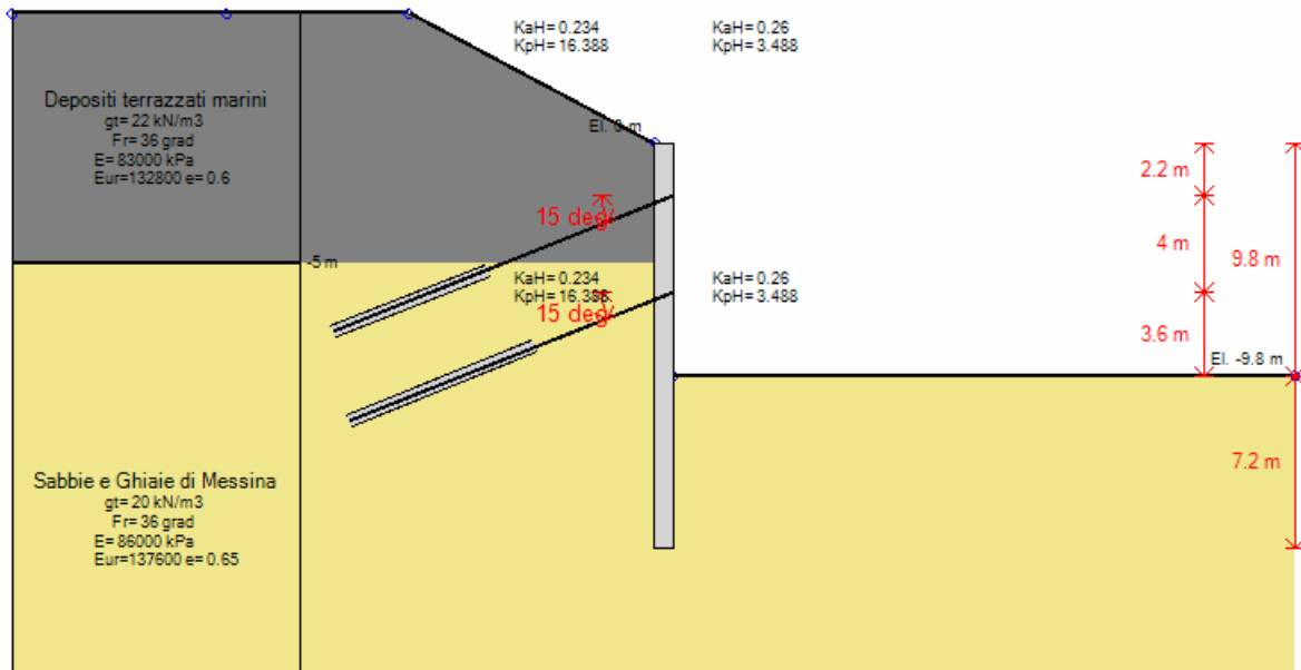
Stage 6 – Sisma
