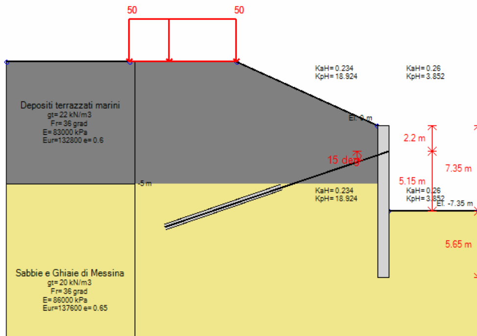
Stage 5 – Sisma
