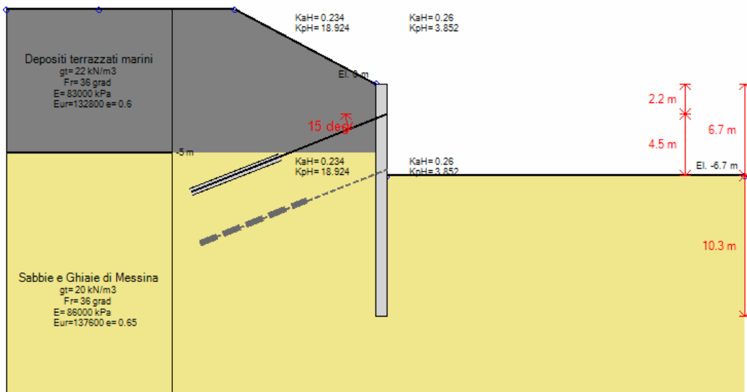
Stage 3 – Scavo a quota -6.70 m
