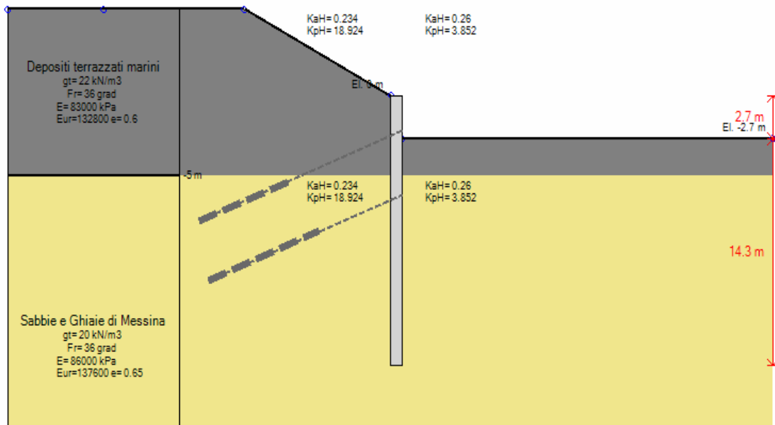
Stage 1 – Scavo a quota -2.70 m
