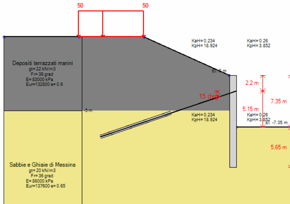
Stage 4 – Scavo a quota -7.35 m
