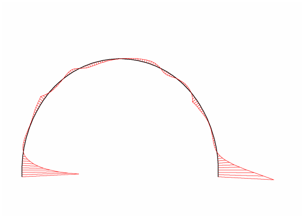
Fig. 15 Shear forces in beam Extreme value -174.63 \cdot 10^{-15} kN/m (Phase: 2)
