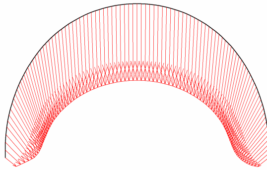
Fig. 66 Total displacements in beam Extreme value 76.08 \cdot 10^{-3} m (Phase: 8)
