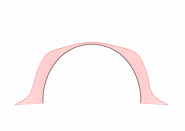
Fig. 78 Bending moments in beam Extreme value -140.95 kNm/m (Phase: 6)
