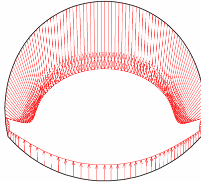
Fig. 55 Total displacements in beam Extreme value 75.81 \cdot 10^{-3} m (Phase: 7)
