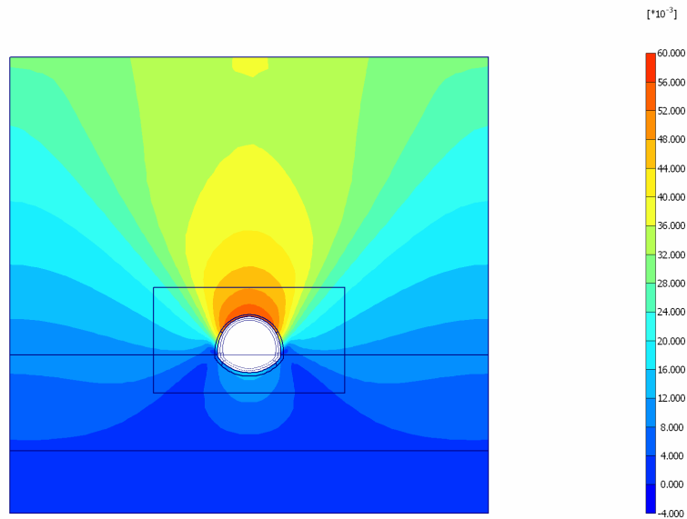
Fig. 3 Plot of total displacements (shadings) - Step no: 12 - ( Phase: 2 )
