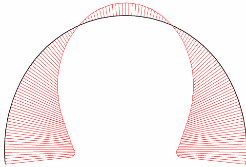
Fig. 86 Axial forces in beam Extreme value -16.17 \cdot 10^{-9} kN/m (Phase: 7)
