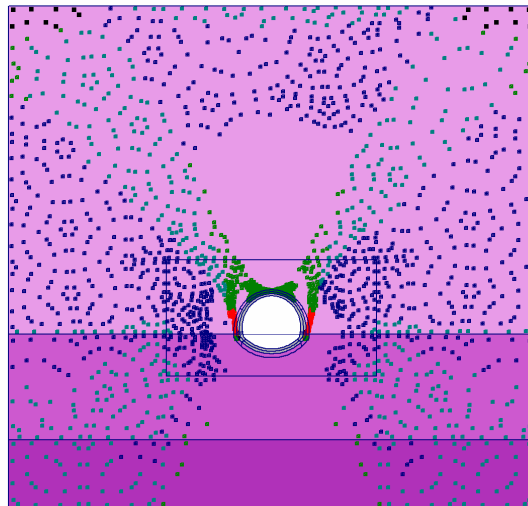
Fig. 7 Plot of plastic points - Step no: 27 - ( Phase: 7 )
