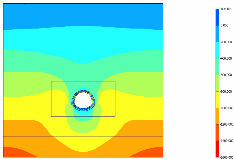
Fig. 64 Plot of effective stresses (mean shadings) - Step no: 31 - ( Phase: 8 )
