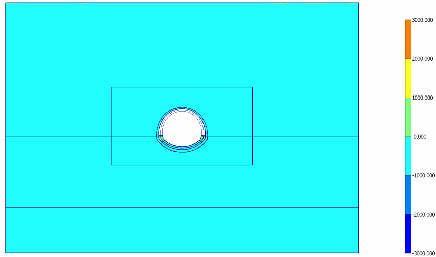
Fig. 54 Plot of effective stresses (mean shadings) - Step no: 20 - ( Phase: 6 )
