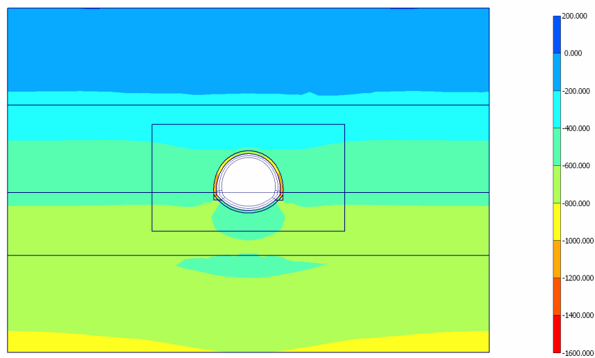
Fig. 21 Plot of effective stresses (mean shadings) - Step no: 9 - ( Phase: 3 )
