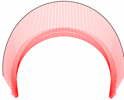
Fig. 83 Total displacements in beam Extreme value 135.43 \cdot 10^{-3} m (Phase: 7)
