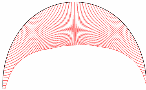
Fig. 57 Axial forces in beam Extreme value -939.51 kN/m (Phase: 5)
