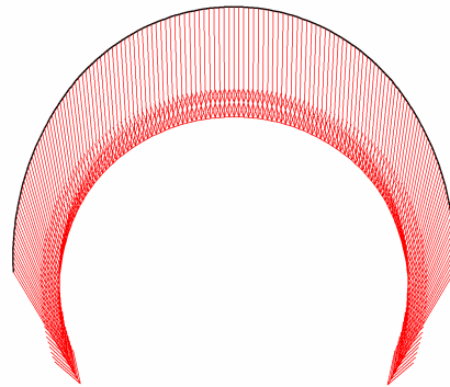
Fig. 84 Total displacements in beam Extreme value 155.48 \cdot 10^{-3} m (Phase: 7)
