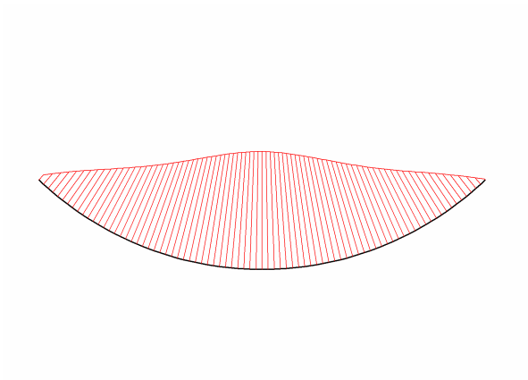
Fig. 106 Bending moments in beam Extreme value 36.48 \cdot 10^{-9} kNm/m (Phase: 8)
