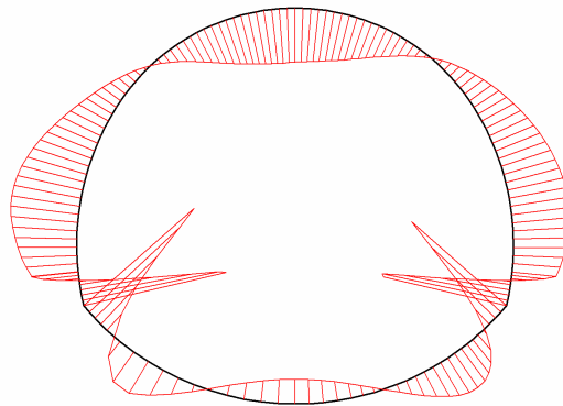
Fig. 61 Bending moments in beam Extreme value 4.53 \cdot 10^{-9} kNm/m (Phase: 7)
