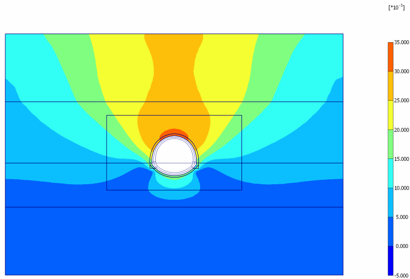
Fig. 20 Plot of total displacements (shadings) - Step no: 9 - ( Phase: 3 )
