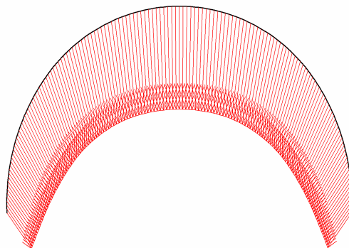
Fig. 9 Total displacements in beam Extreme value 15.45 \cdot 10^{-3} m (Phase: 2)
