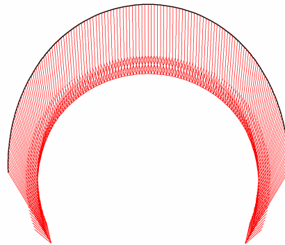
Fig. 69 Total displacements in beam Extreme value 154.36 \cdot 10^{-3} m (Phase: 6)
