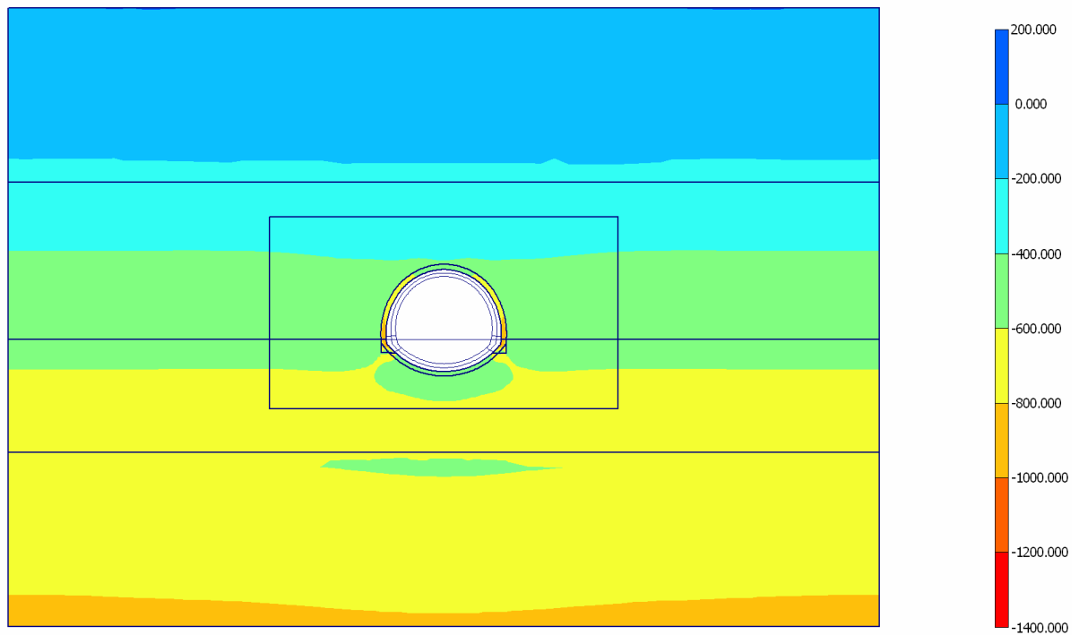
Fig. 6 Plot of effective stresses (mean shadings) - Step no: 6 - ( Phase: 2 )
