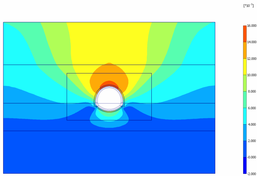
Fig. 5 Plot of total displacements (shadings) - Step no: 6 - ( Phase: 2 )
