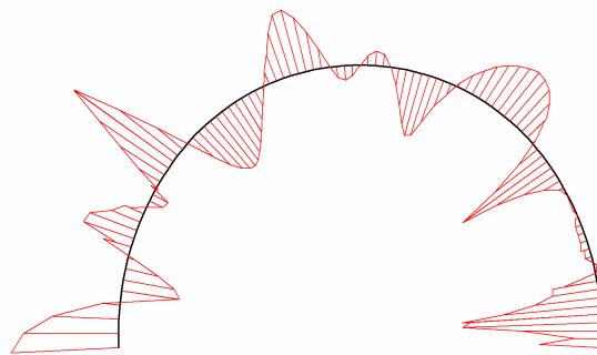
Fig. 30 Shear forces in beam Extreme value -9.02 kN/m (Phase: 4)
