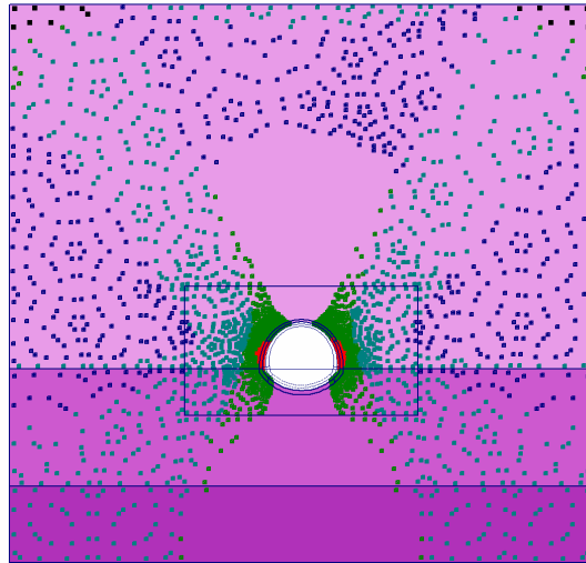
Fig. 3 Plot of plastic points - Step no: 15 - ( Phase: 3 )
