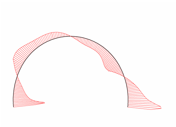
Fig. 104 Shear forces in beam Extreme value 17.38 \cdot 10^{-9} kN/m (Phase: 8)
