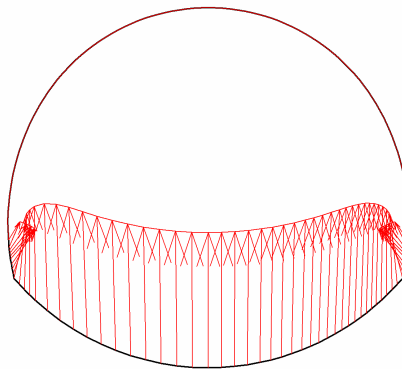
Fig. 45 Total displacements in beam Extreme value 18.17 \cdot 10^{-3} m (Phase: 6)
