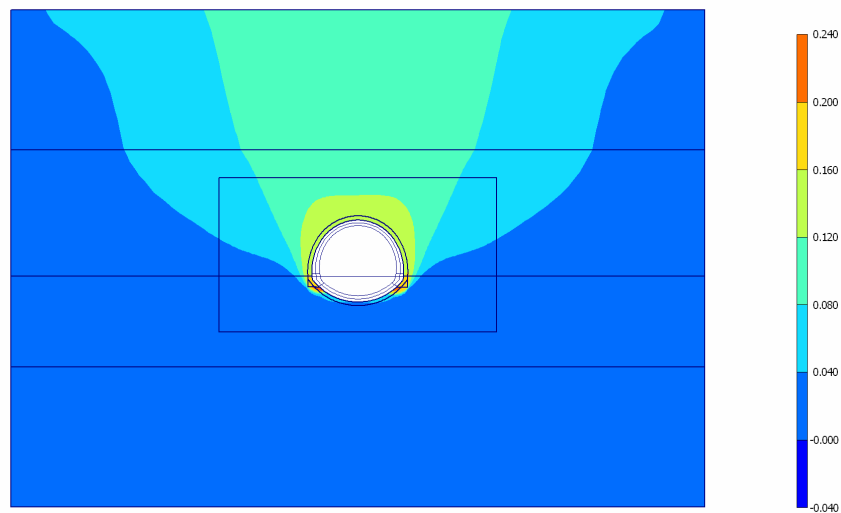
Fig. 50 Plot of total displacements (shadings) - Step no: 83 - ( Phase: 5 )
