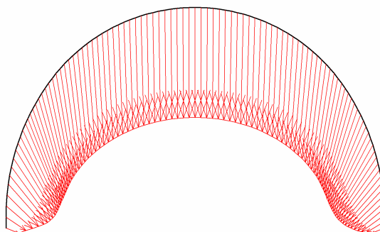
Fig. 26 Total displacements in beam Extreme value 70.74 \cdot 10^{-3} m (Phase: 4)
