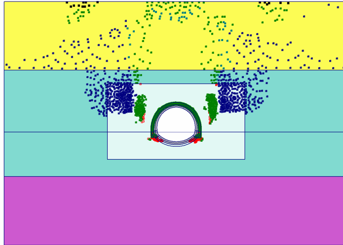
Fig. 8 Plot of plastic points
