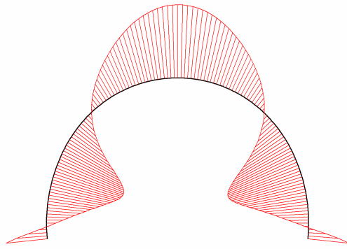
Fig. 107 Bending moments in beam Extreme value 14.67 \cdot 10^{-9} kNm/m (Phase: 8)
