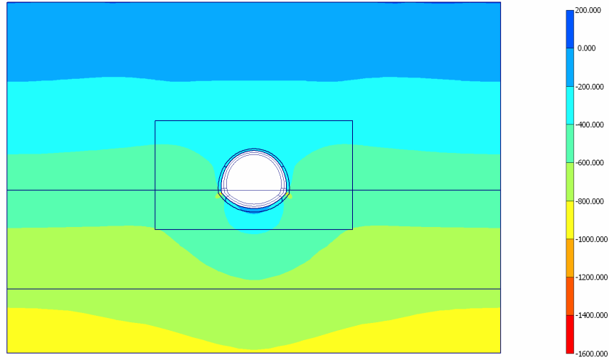
Fig. 34 Plot of effective stresses (mean shadings) - Step no: 13 - ( Phase: 4 )
