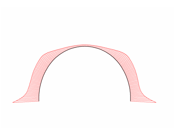
Fig. 92 Bending moments in beam Extreme value -5.96 \cdot 10^{-9} kNm/m (Phase: 7)
