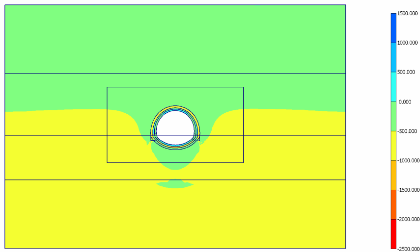
Fig. 81 Plot of effective stresses (mean shadings) - Step no: 90 - ( Phase: 7 )
