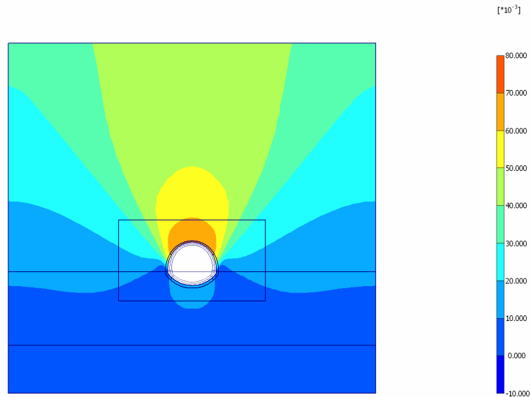
Fig. 23 Plot of total displacements (shadings) - Step no: 19 - ( Phase: 4 )
