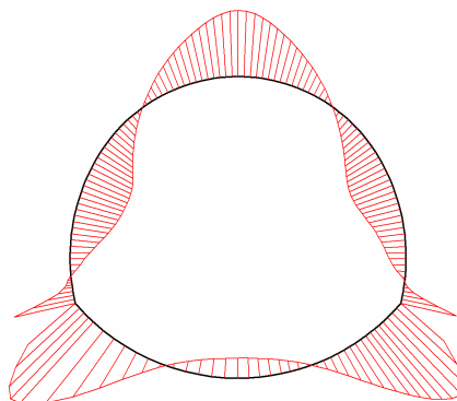
Fig. 71 Bending moments in beam Extreme value -19.11 \cdot 10^{-9} kNm/m (Phase: 8)
