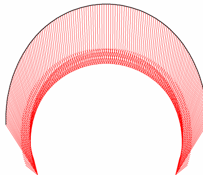
Fig. 39 Total displacements in beam Extreme value 70.73 \cdot 10^{-3} m (Phase: 4)
