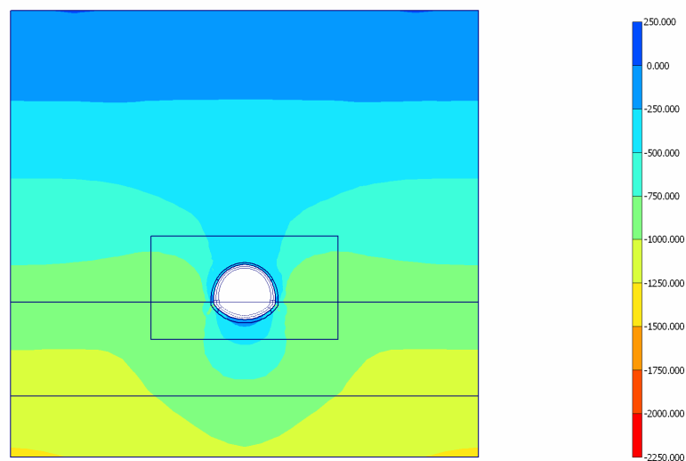
Fig. 34 Plot of effective stresses (mean shadings) - Step no: 23 - ( Phase: 5 )
