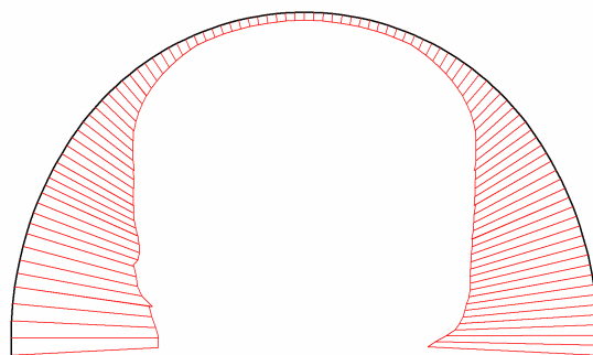
Fig. 8 Axial forces in beam Extreme value -14.17 \cdot 10^{-12} kN/m (Phase: 2)
