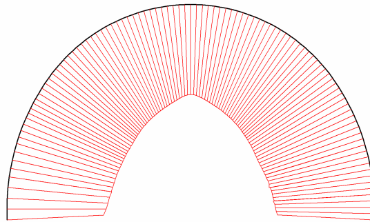
Fig. 58 Axial forces in beam Extreme value -1.13 \cdot 10^3 kN/m (Phase: 7)
