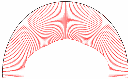
Fig. 72 Axial forces in beam Extreme value -1.27 \cdot 10^3 kN/m (Phase: 6)
