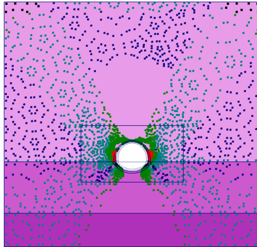
Fig. 5 Plot of plastic points - Step no: 23 - ( Phase: 5 )
