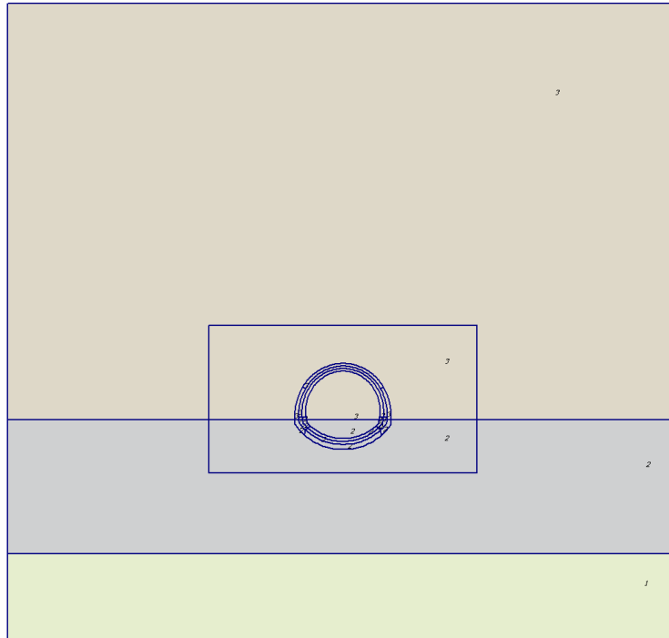
Fig. 2 Plot of geometry with material data sets
