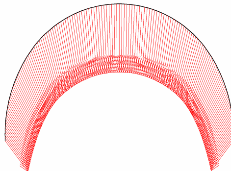
Fig. 24 Total displacements in beam Extreme value 32.20 \cdot 10^{-3} m (Phase: 3)
