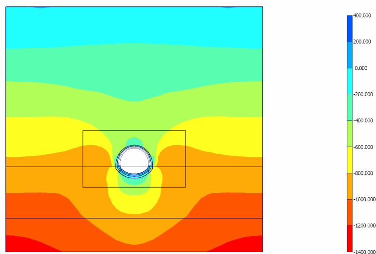
Fig. 44 Plot of effective stresses (mean shadings) - Step no: 25 - ( Phase: 6 )
