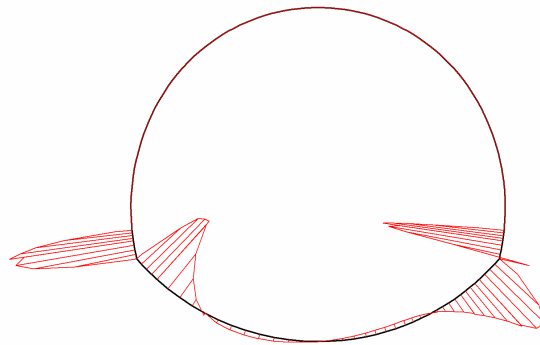
Fig. 49 Shear forces in beam Extreme value 8.69 \cdot 10^{-9} kN/m (Phase: 6)
