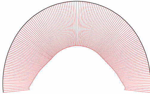
Fig. 101 Axial forces in beam Extreme value -218.37 \cdot 10^{-9} kN/m (Phase: 8)
