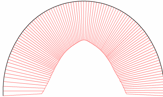
Fig. 38 Axial forces in beam Extreme value -1.11 \cdot 10^3 kN/m (Phase: 5)
