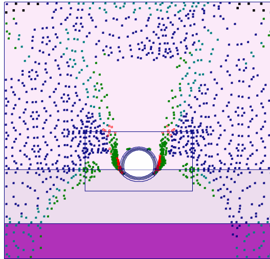
Fig. 8 Plot of plastic points - Step no: 31 - ( Phase: 8 )
