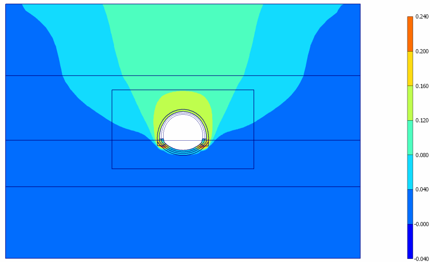
Fig. 65 Plot of total displacements (shadings) - Step no: 88 - ( Phase: 6 )
