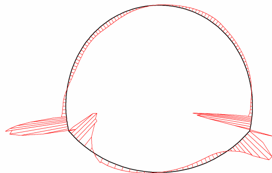
Fig. 59 Shear forces in beam Extreme value 9.43 \cdot 10^{-9} kN/m (Phase: 7)
