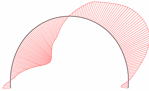
Fig. 89 Shear forces in beam Extreme value -1.79 \cdot 10^{-9} kN/m (Phase: 7)
