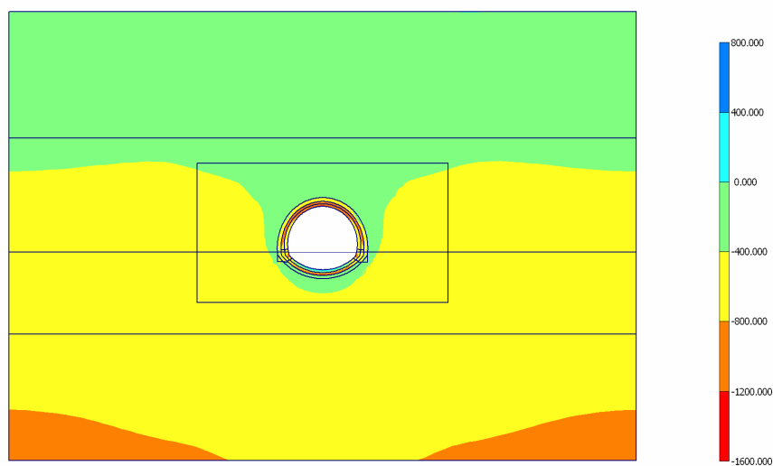
Fig. 96 Plot of effective stresses (mean shadings) - Step no: 96 - ( Phase: 8 )
