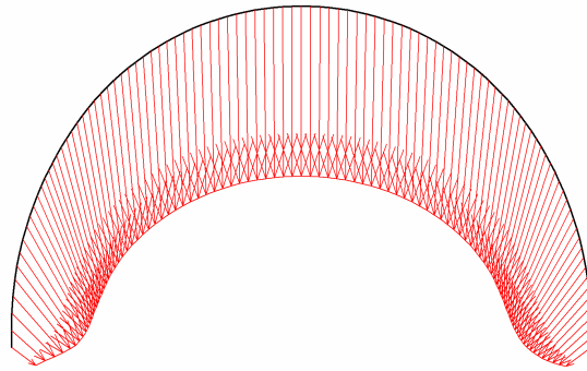
Fig. 46 Total displacements in beam Extreme value 75.18 \cdot 10^{-3} m (Phase: 6)
