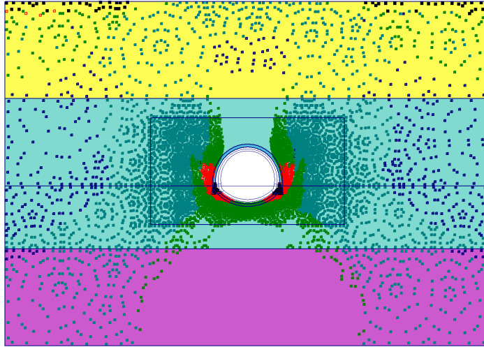
Fig. 5 Plot of plastic points - Step no: 83 - ( Phase: 5 )
