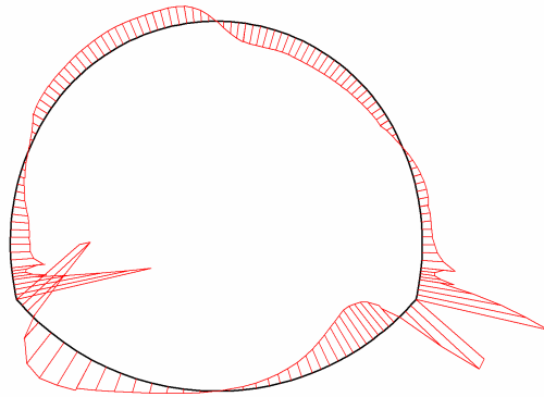
Fig. 69 Shear forces in beam Extreme value -25.20 \cdot 10^{-9} kN/m (Phase: 8)
