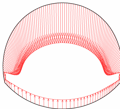
Fig. 65 Total displacements in beam Extreme value 76.07 \cdot 10^{-3} m (Phase: 8)
