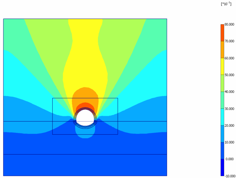
Fig. 63 Plot of total displacements (shadings) - Step no: 31 - ( Phase: 8 )
