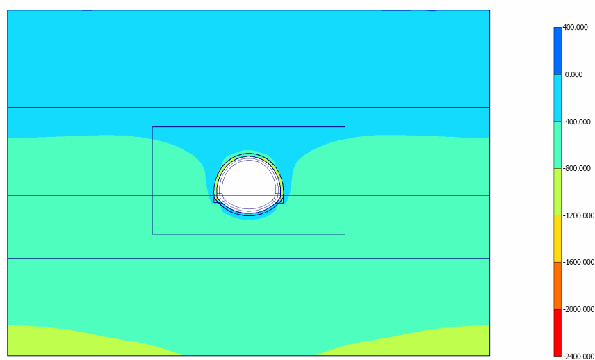
Fig. 36 Plot of effective stresses (mean shadings) - Step no: 53 - ( Phase: 4 )
