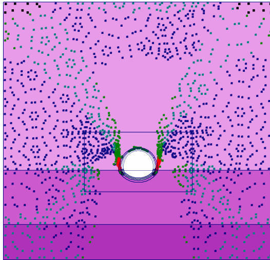
Fig. 6 Plot of plastic points - Step no: 25 - ( Phase: 6 )
