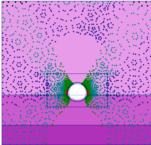
Fig. 2 Plot of plastic points - Step no: 12 - ( Phase: 2 )
