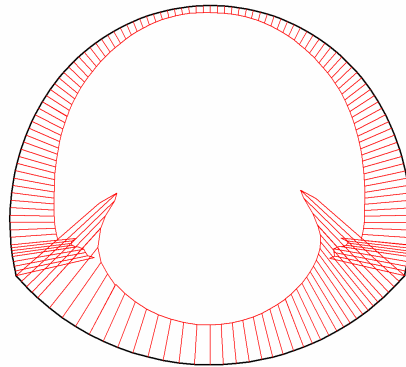
Fig. 57 Axial forces in beam Extreme value -38.34 \cdot 10^{-9} kN/m (Phase: 7)
