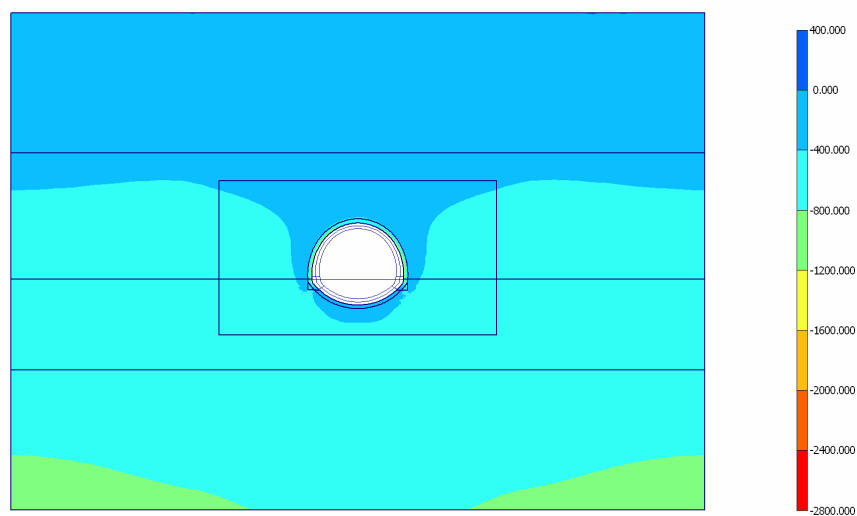
Fig. 51 Plot of effective stresses (mean shadings) - Step no: 83 - ( Phase: 5 )
