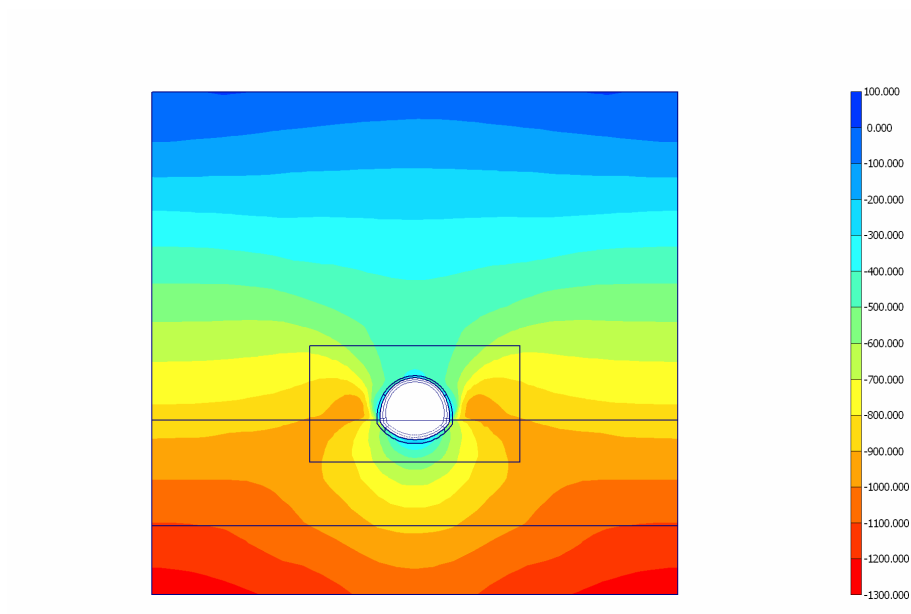
Fig. 14 Plot of effective stresses (mean shadings) - Step no: 15 - ( Phase: 3 )
