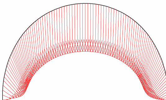
Fig. 16 Total displacements in beam Extreme value 65.42 \cdot 10^{-3} m (Phase: 3)
