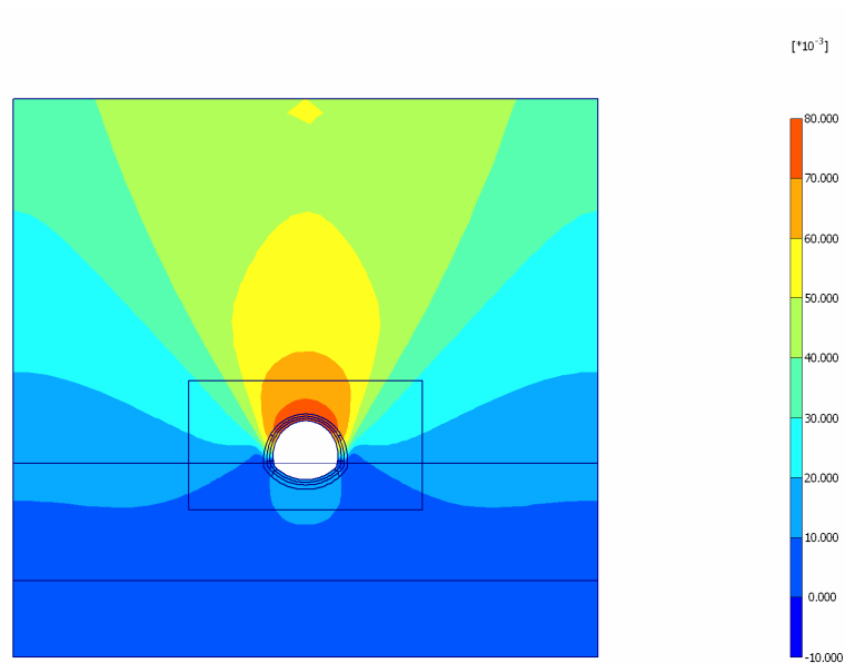
Fig. 53 Plot of total displacements (shadings) - Step no: 27 - ( Phase: 7 )
