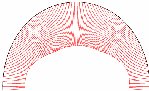
Fig. 87 Axial forces in beam Extreme value -1.32 \cdot 10^3 kN/m (Phase: 7)
