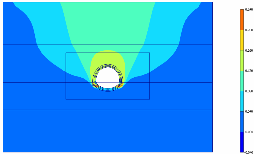
Fig. 95 Plot of total displacements (shadings) - Step no: 96 - ( Phase: 8 )
