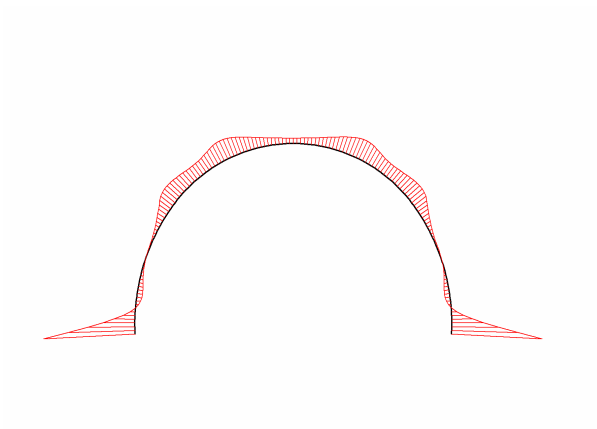
Fig. 18 Bending moments in beam Extreme value -88.51 \cdot 10^{-15} kNm/m (Phase: 2)
