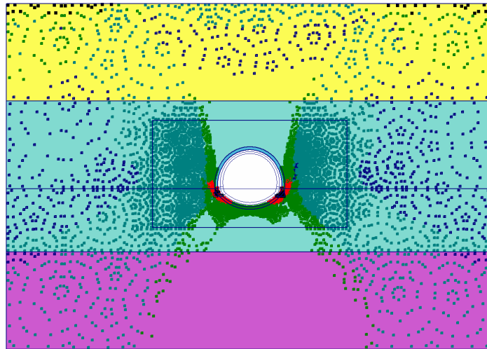
Fig. 4 Plot of plastic points - Step no: 53 - ( Phase: 4 )
