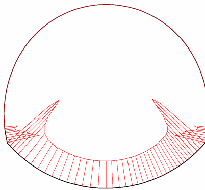
Fig. 47 Axial forces in beam Extreme value -27.78 \cdot 10^{-9} kN/m (Phase: 6)
