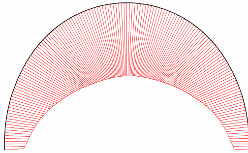
Fig. 42 Axial forces in beam Extreme value -766.54 kN/m (Phase: 4)
