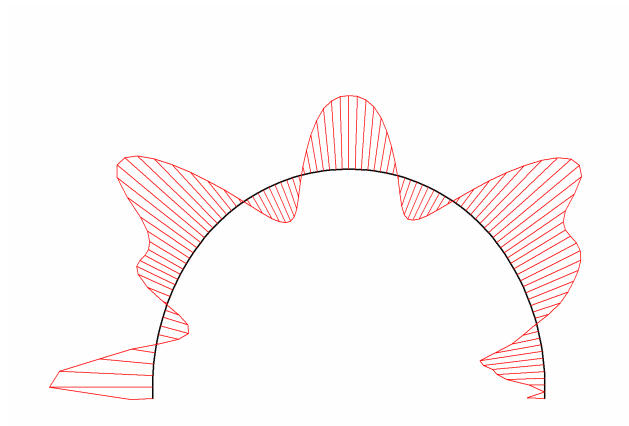
Fig. 52 Bending moments in beam Extreme value -8.03 kNm/m (Phase: 6)
