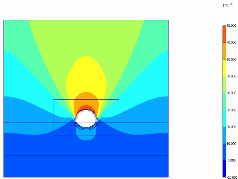
Fig. 43 Plot of total displacements (shadings) - Step no: 25 - ( Phase: 6 )
