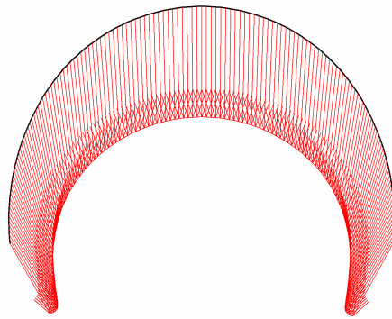
Fig. 98 Total displacements in beam Extreme value 137.56 \cdot 10^{-3} m (Phase: 8)
