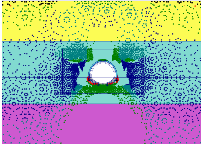
Fig. 6 Plot of plastic points - Step no: 88 - ( Phase: 6 )
