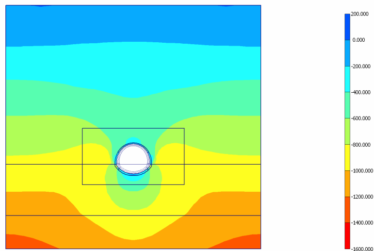
Fig. 24 Plot of effective stresses (mean shadings) - Step no: 19 - ( Phase: 4 )
