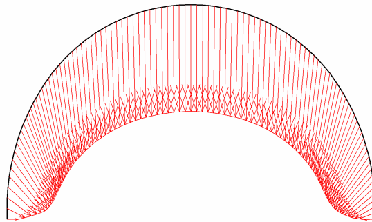
Fig. 6 Total displacements in beam Extreme value 56.24 \cdot 10^{-3} m (Phase: 2)
