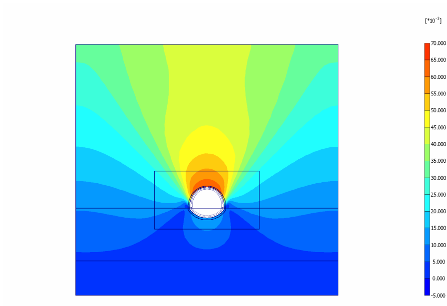
Fig. 13 Plot of total displacements (shadings) - Step no: 15 - ( Phase: 3 )
