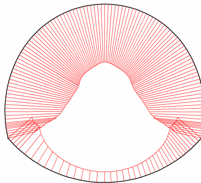
Fig. 67 Axial forces in beam Extreme value -166.44 \cdot 10^{-9} kN/m (Phase: 8)
