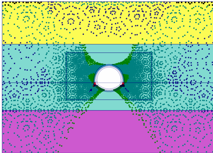
Fig. 3 Plot of plastic points - Step no: 9 - ( Phase: 3 )
