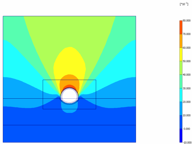
Fig. 33 Plot of total displacements (shadings) - Step no: 23 - ( Phase: 5 )
