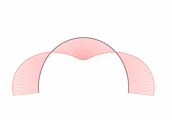
Fig. 92 Bending moments in beam Extreme value -5.96 \cdot 10^{-9} kNm/m (Phase: 7)
