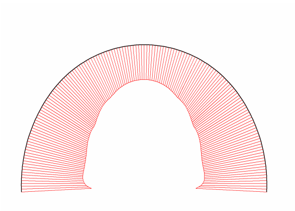
Fig. 12 Axial forces in beam Extreme value -1.56 \cdot 10^{-12} kN/m (Phase: 2)
