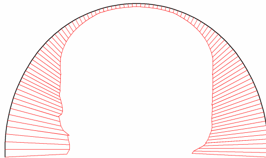
Fig. 18 Axial forces in beam Extreme value -16.94 \cdot 10^{-12} kN/m (Phase: 3)
