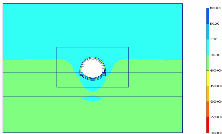
Fig. 66 Plot of effective stresses (mean shadings) - Step no: 88 - ( Phase: 6 )
