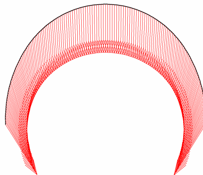
Fig. 54 Total displacements in beam Extreme value 154.93 \cdot 10^{-3} m (Phase: 5)
