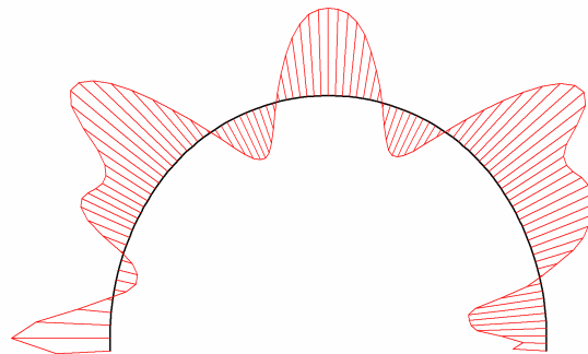
Fig. 42 Bending moments in beam Extreme value -7.64 kNm/m (Phase: 5)
