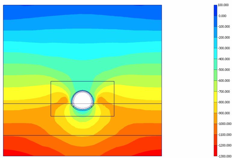
Fig. 4 Plot of effective stresses (mean shadings) - Step no: 12 - ( Phase: 2 )
