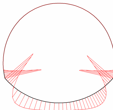
Fig. 51 Bending moments in beam Extreme value 5.71 \cdot 10^{-9} kNm/m (Phase: 6)
