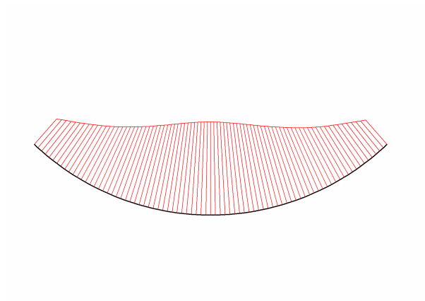
Fig. 76 Bending moments in beam Extreme value 35.78 \cdot 10^{-9} kNm/m (Phase: 6)
