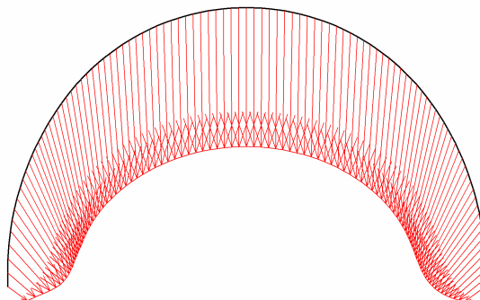
Fig. 36 Total displacements in beam Extreme value 74.81 \cdot 10^{-3} m (Phase: 5)
