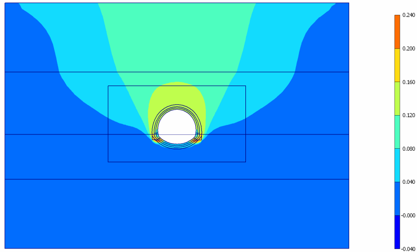
Fig. 80 Plot of total displacements (shadings) - Step no: 90 - ( Phase: 7 )
