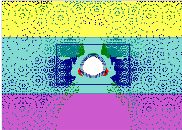
Fig. 7 Plot of plastic points - Step no: 90 - ( Phase: 7 )
