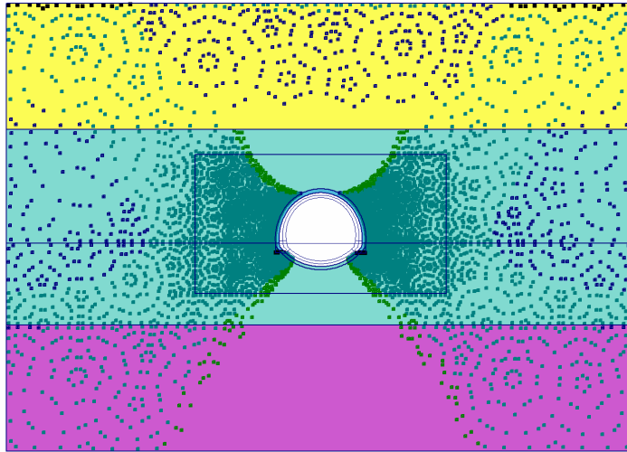
Fig. 2 Plot of plastic points - Step no: 6 - ( Phase: 2 )
