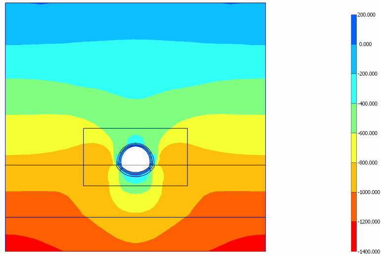
Fig. 54 Plot of effective stresses (mean shadings) - Step no: 27 - ( Phase: 7 )
